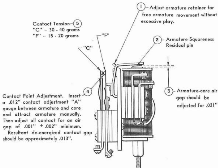
Figure 10. X-R, MCR of Type 405
