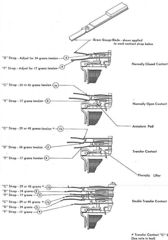
Figure 6. Contact Strap Tension
