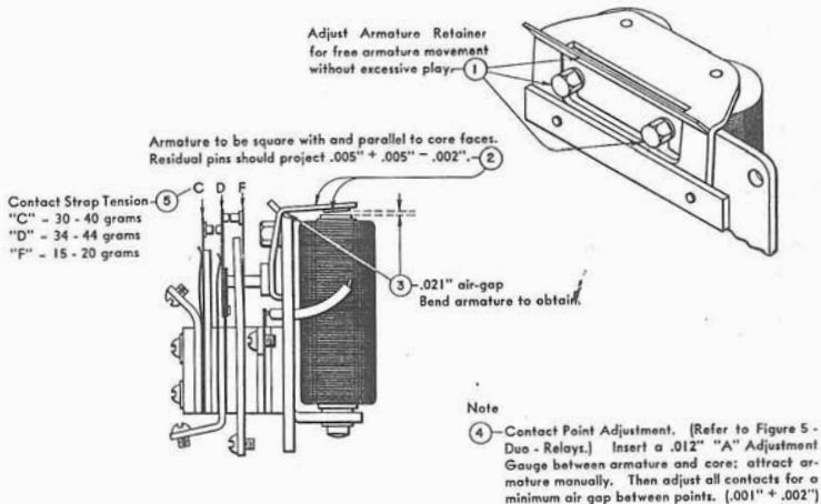
Figure 9. Multi-Contact Relay
