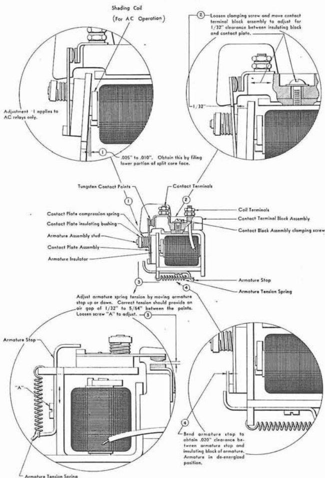
Figure 14. IBM Unit Type Relay
