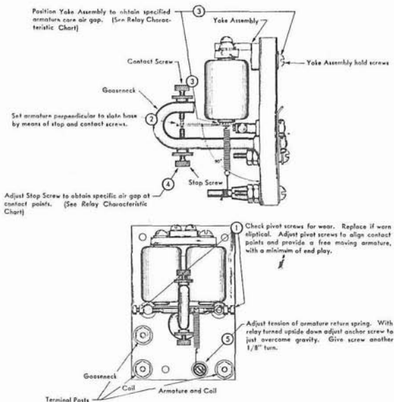
Figure 12. Slate Base Relay
