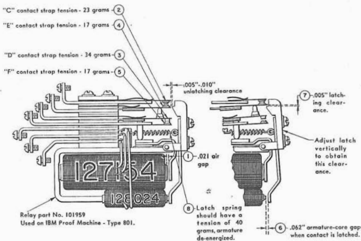
Figure 8. Duo Latch Relay Adjustments
