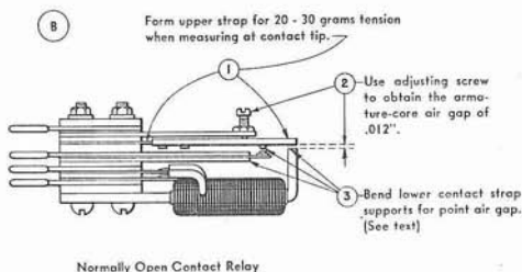
Figure 11. High Speed Relay (Collator)
