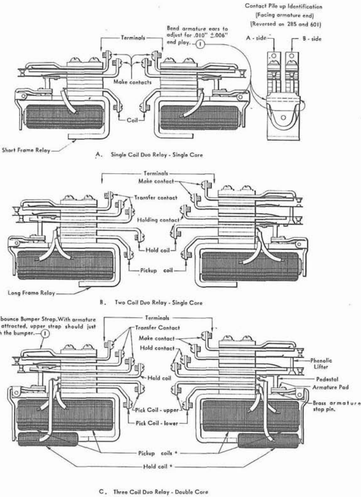
C. Three Coil Duo Relay - Double Core
