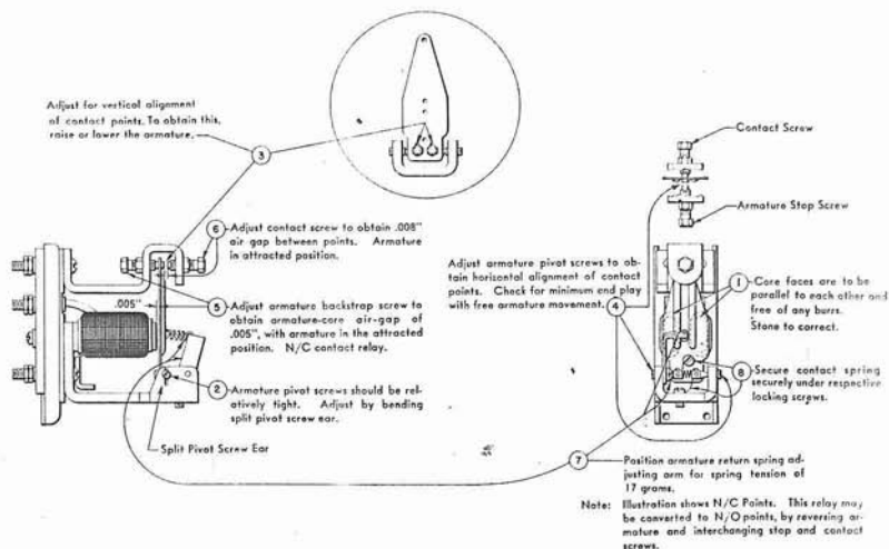
Figure 13. High Speed Relay No. 202800
