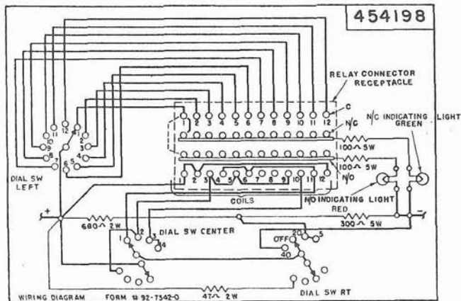
Figure 30B. Testing Device Wiring Diagram
