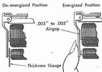
Two Core Relays
