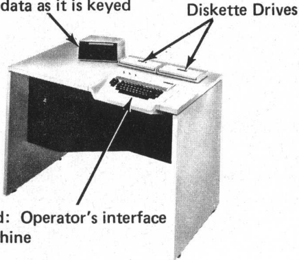
Figure 2. IBM 3741 Data Station (with Second Disk Feature)
