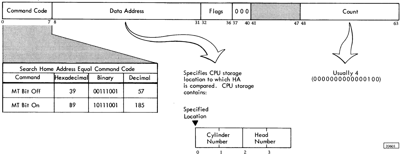
Figure 29. Search Home Address Command
