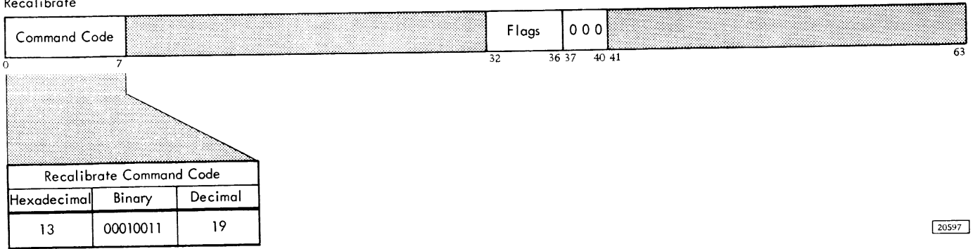
Figure 26. Recalibrate Command
