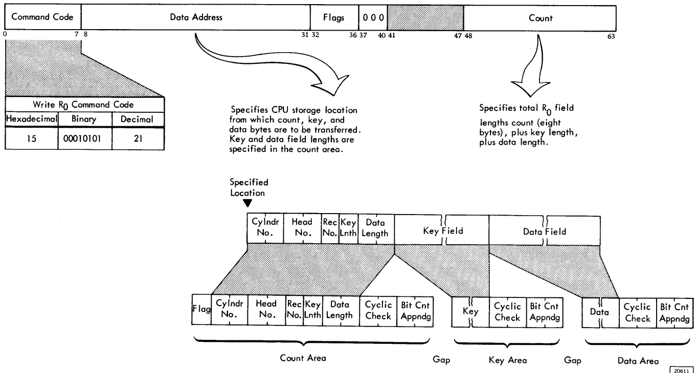
Figure 40. Write Track Descriptor Record (R0) Command
