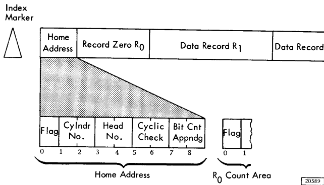
Figure 9. Home Address
