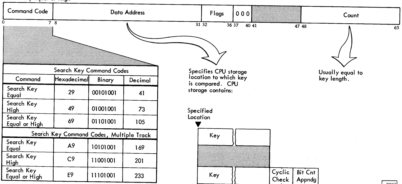
Figure 31. Search Key Commands
