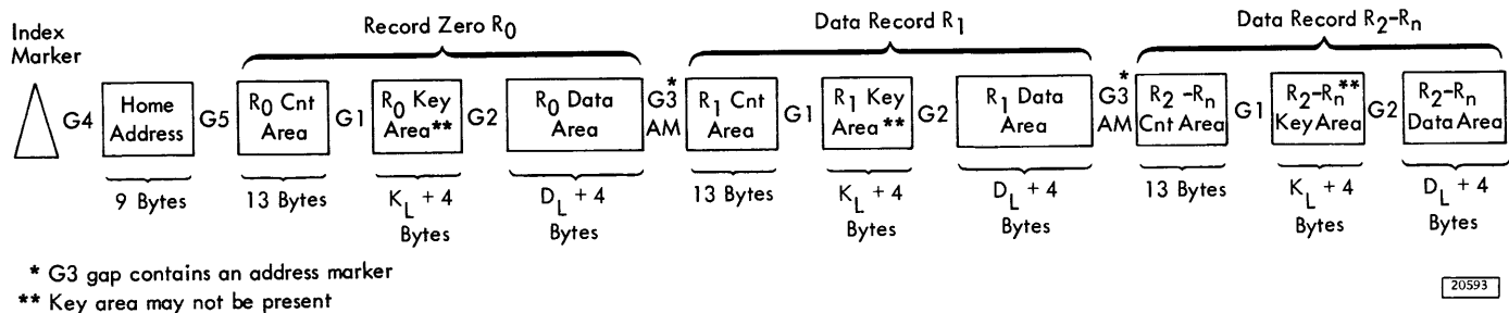
Figure 13. Track Capacity
