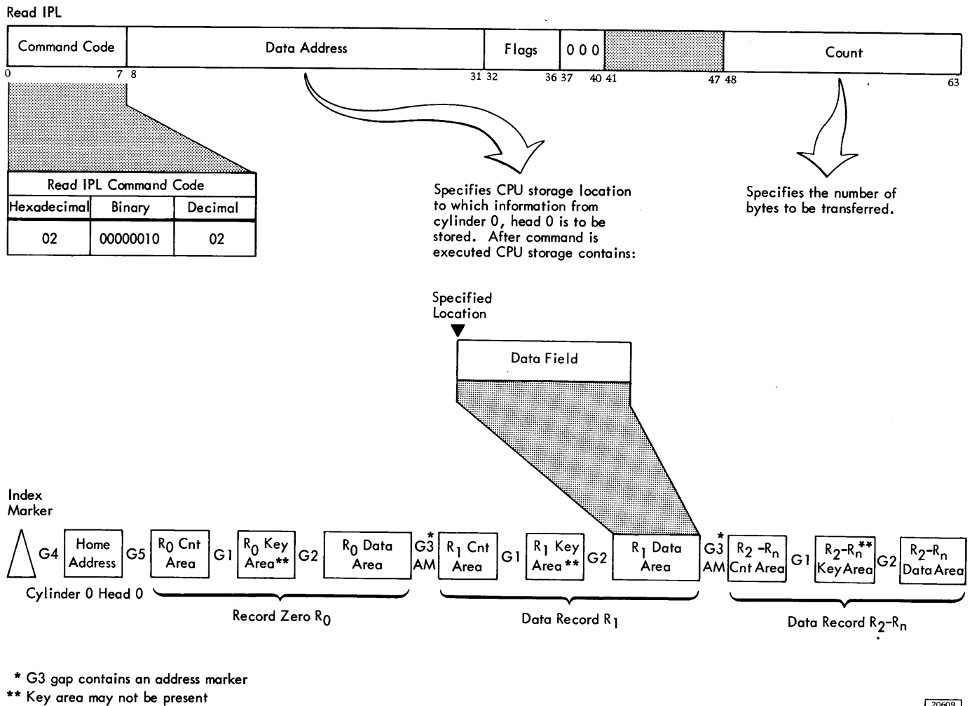
Figure 38. Read Initial Program Load Command
