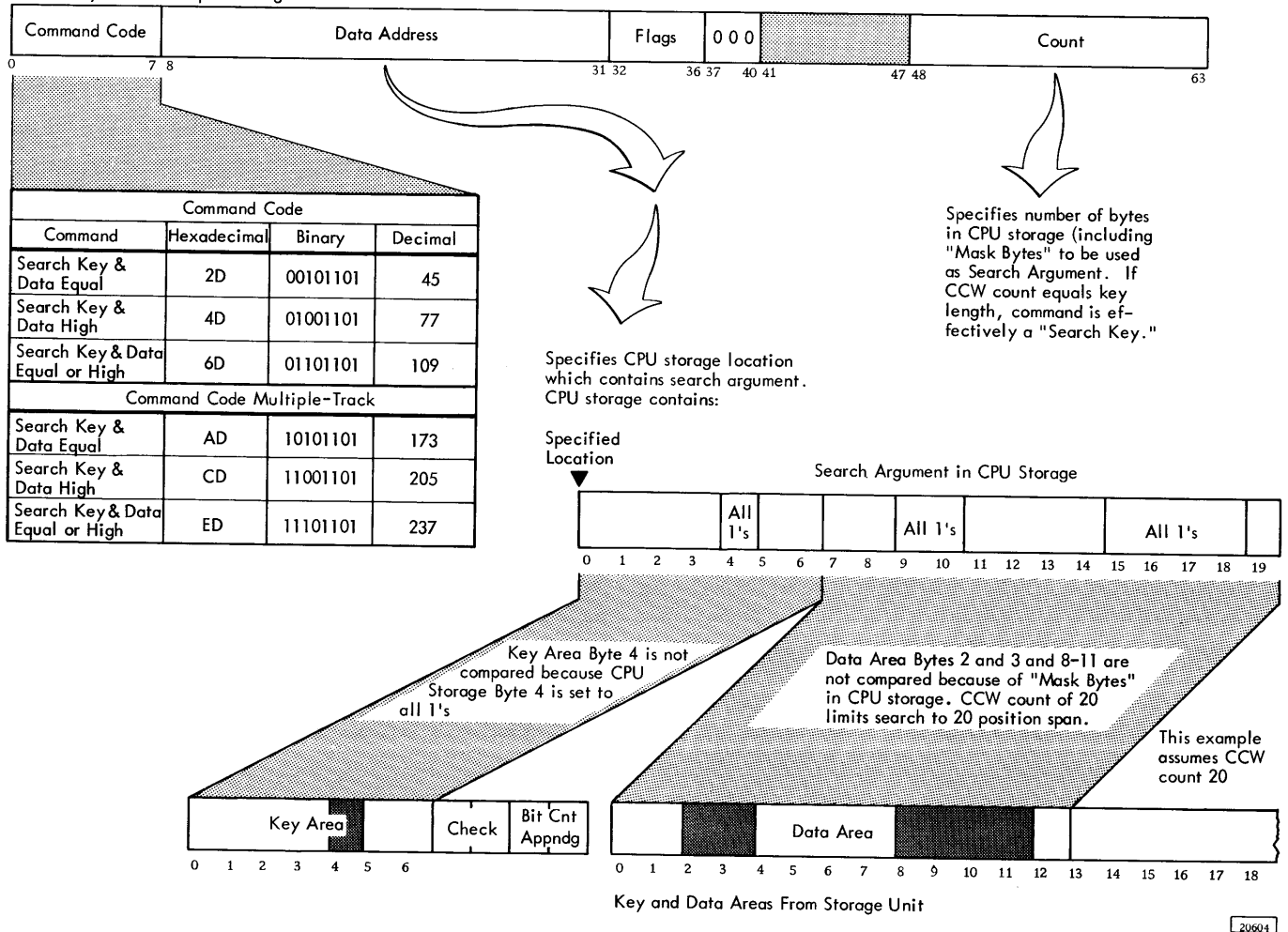
Figure 32. Search Key and Data Commands
