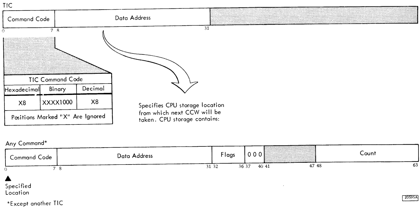
Figure 24. Transfer in Channel Command
