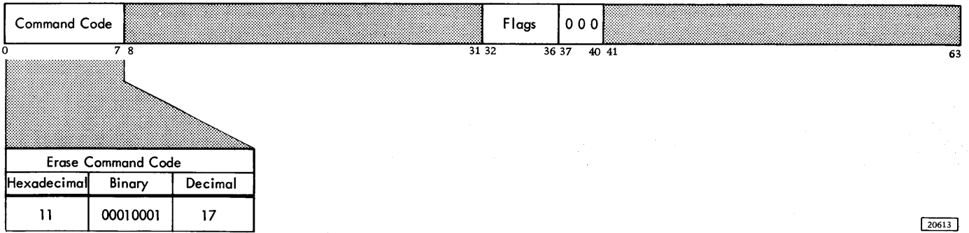
Figure 42. Erase Command
