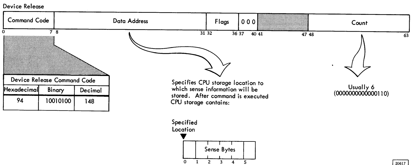
Figure 46. Device Release Command
