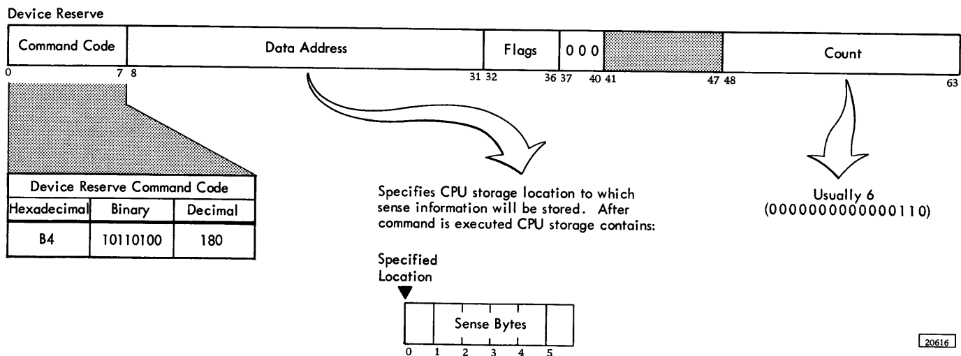
Figure 45. Device Reserve Command
