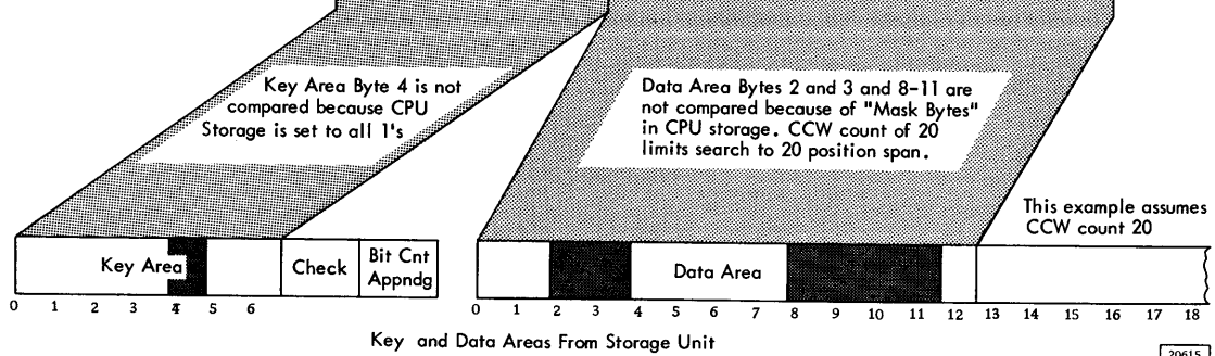
Figure 44. Continue Scan Commands
