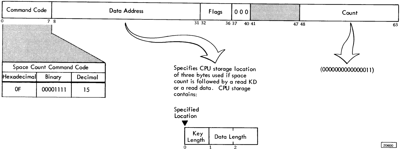
Figure 33. Space Count Command
