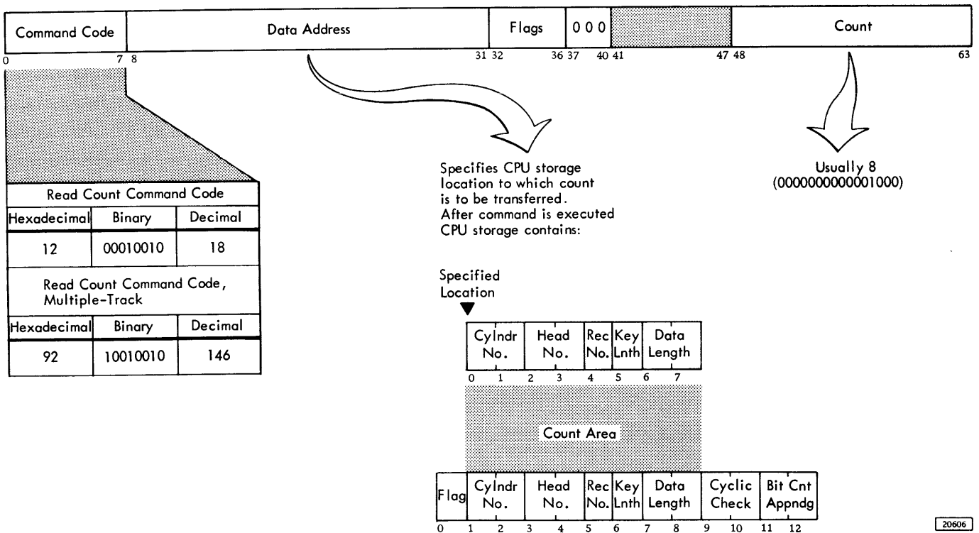
Figure 35. Read Count Command
