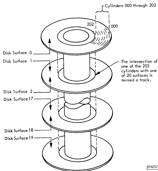
Figure 3. Cylinder Concept
