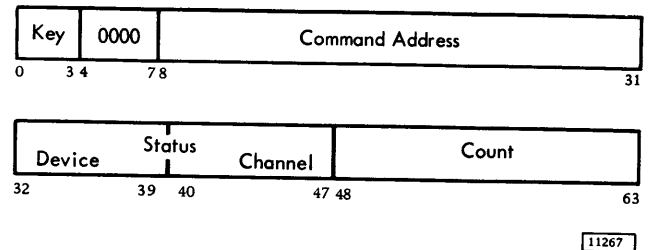
Figure 21. Channel Status Word
