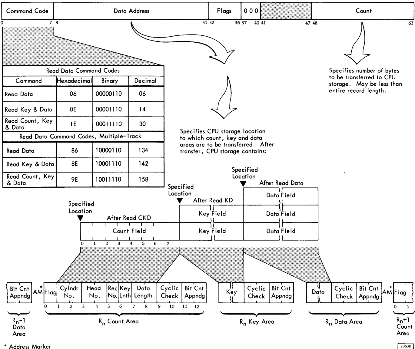
Figure 37. Read Data, Read Key and Data, and Read Count, Key, and Data Commands
