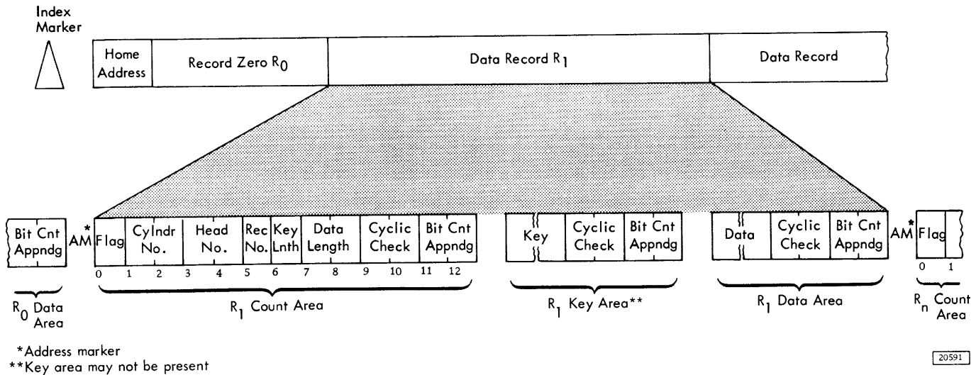
Figure 11. Data Records
