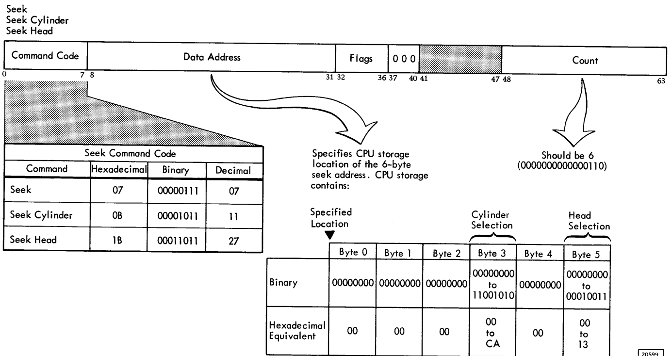
Figure 28. Seek Commands
