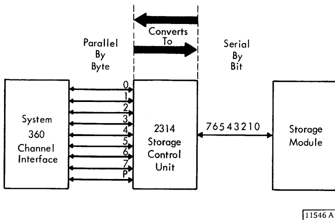
Figure 6. Data Transfer Methods 11546 A
