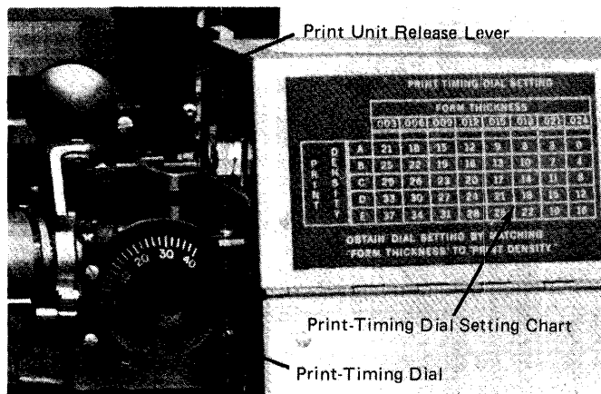
Figure 10. Print-Unit Release Lever (all Models) and Print-Timing Dial, Models 1, 2, 4, 5, 6, 7
