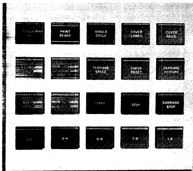
Figure 43. Model N1 Operating Keys and Lights for Selective Tape Listing Feature
