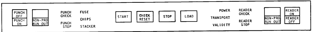
Figure 4. Operating Controls
