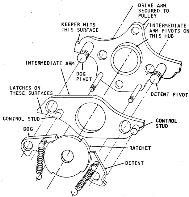
Figure 7. Clutch Operation
