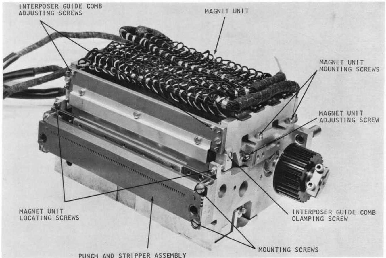
Figure 43. Punch Unit
