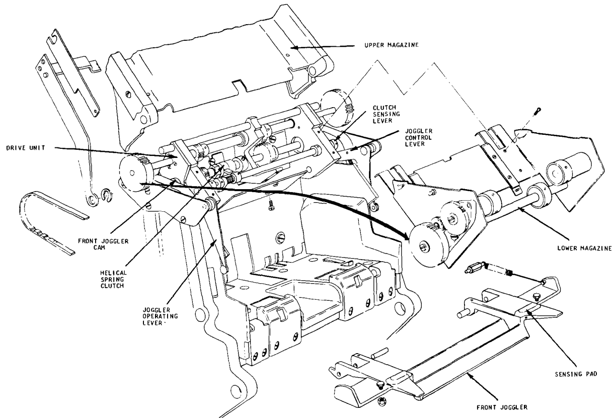
Figure 11. File Feed
