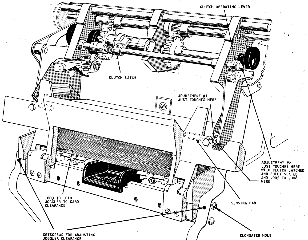
Figure 13. File Feed Adjustments
