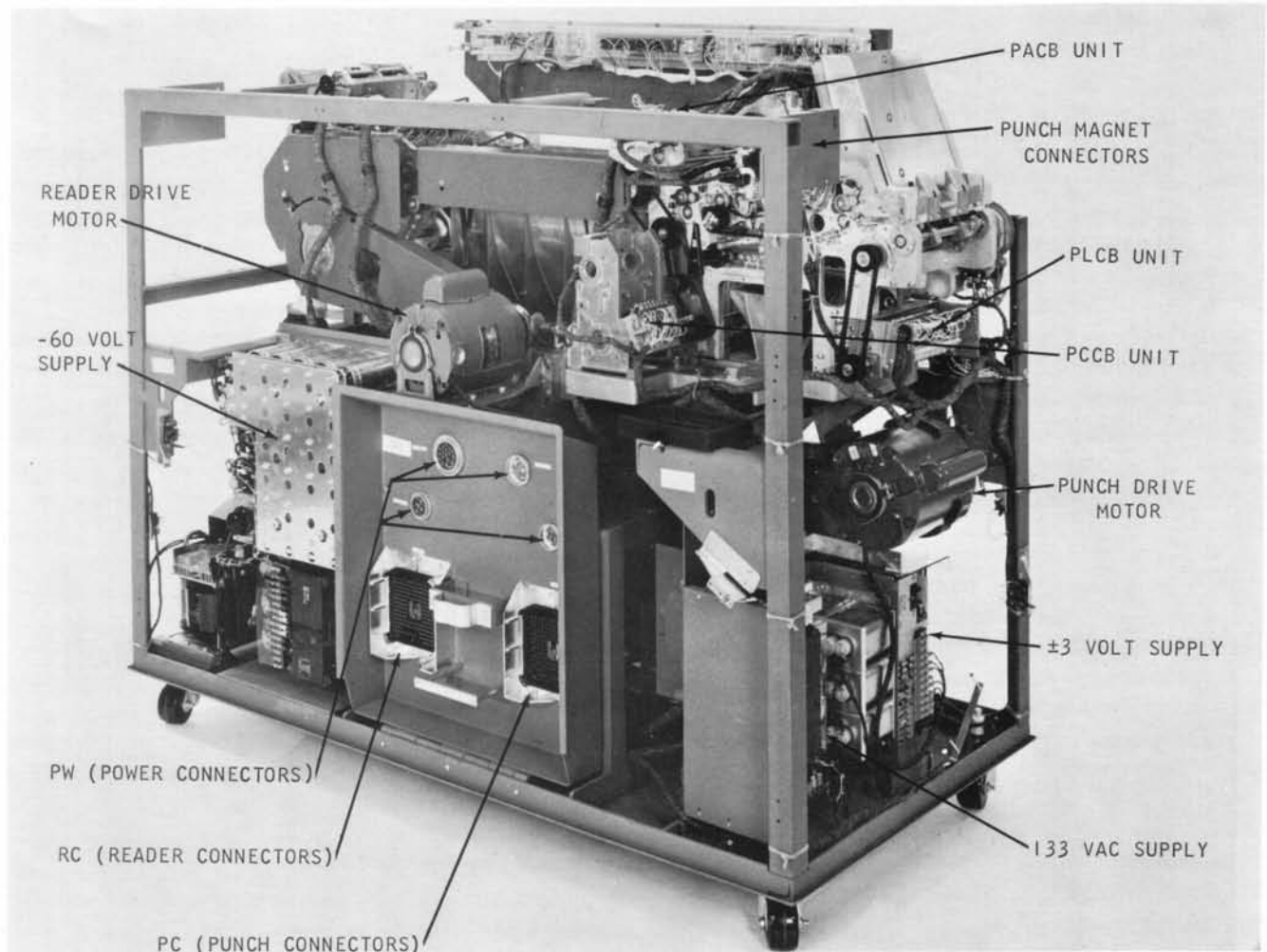
Figure 6. 1402 Rear View
