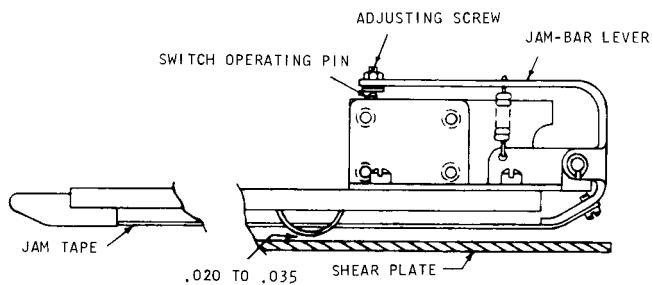
Figure 22. Jam Bar
