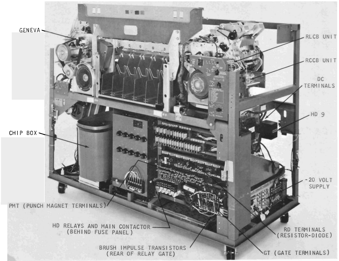
Figure 5. 1402 Front View
