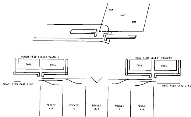
Figure 19. Card Selection Schematic
