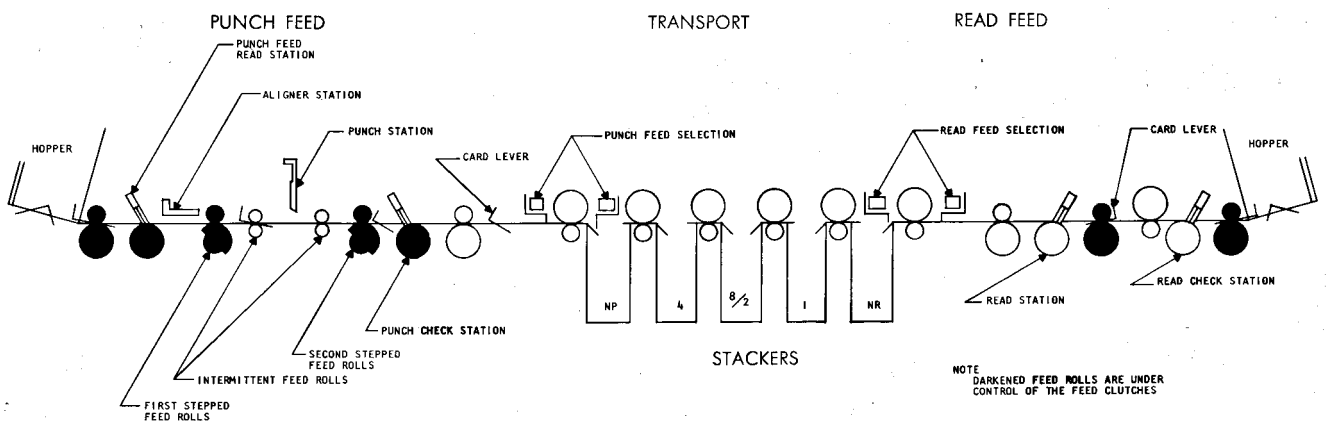
Figure 1. 1402 Feed Schematic
