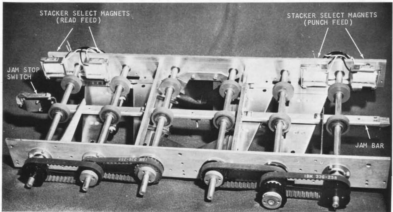
Figure 2. Transport Mechanism
