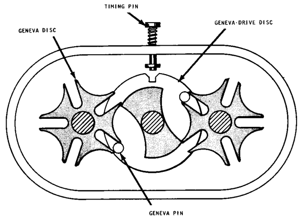
Figure 35. Geneva
