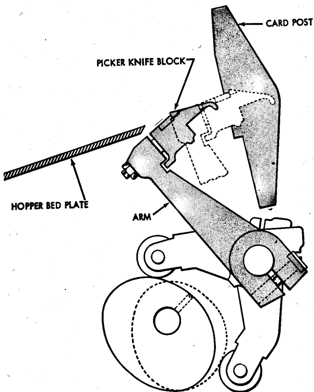
Figure 16. Picker Knives
