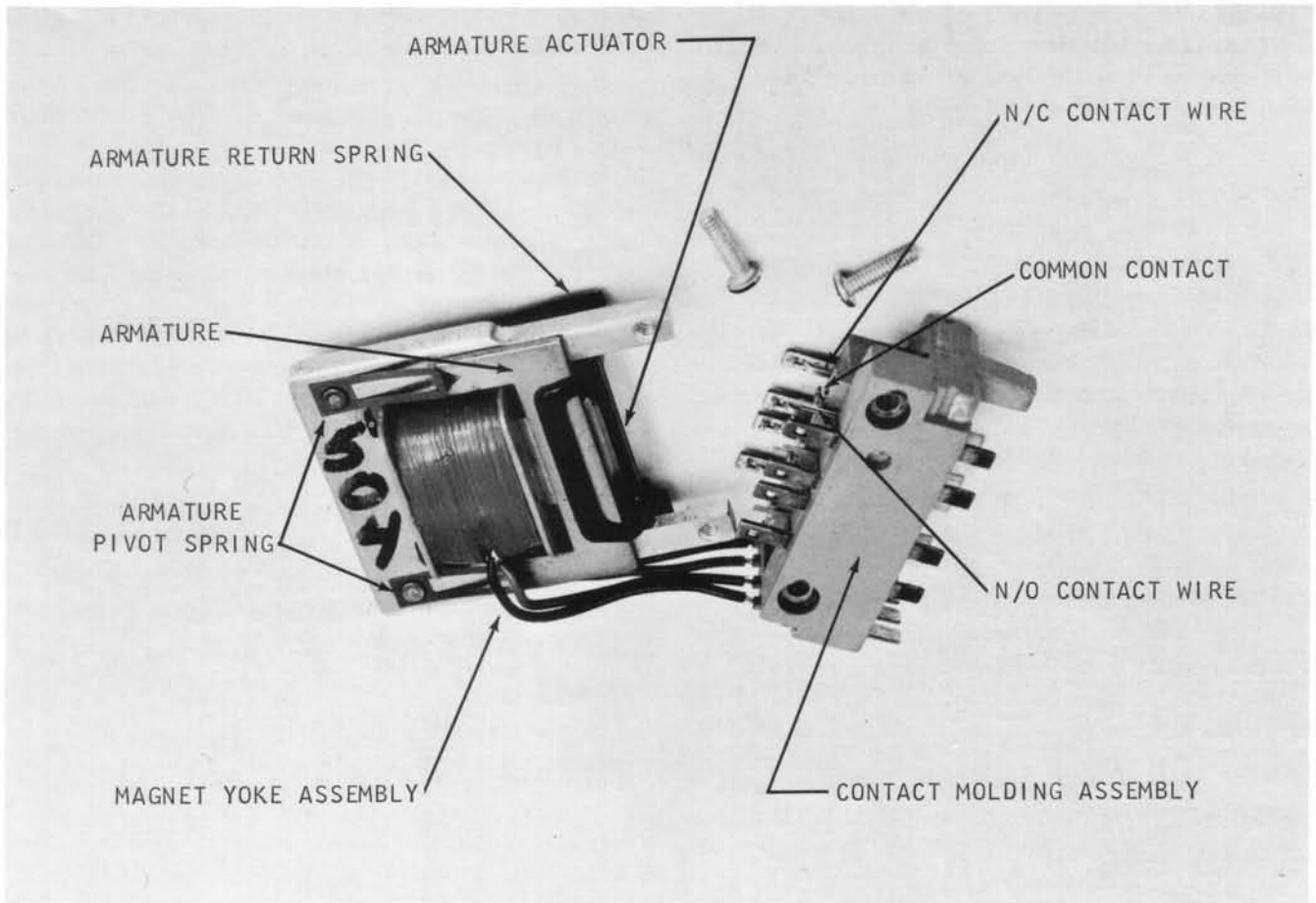
Figure 52. PM Relay
