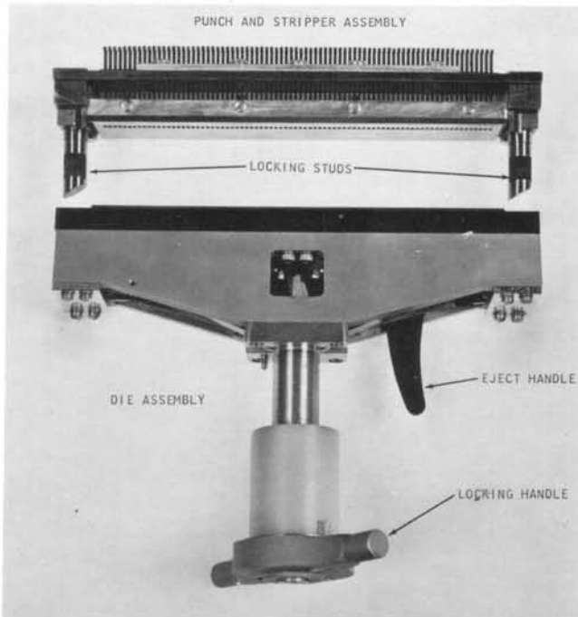
Figure 48. Redesigned Die and Stripper
