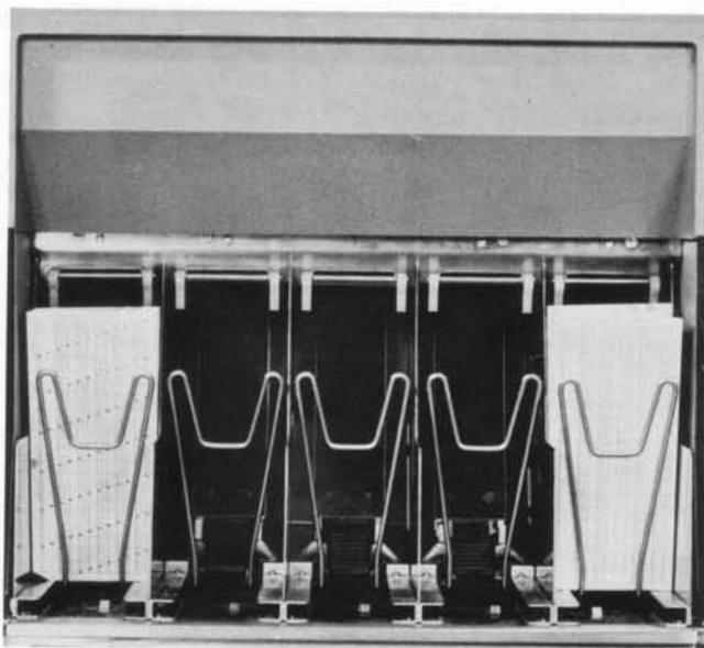
Figure 3. Radial Stackers
