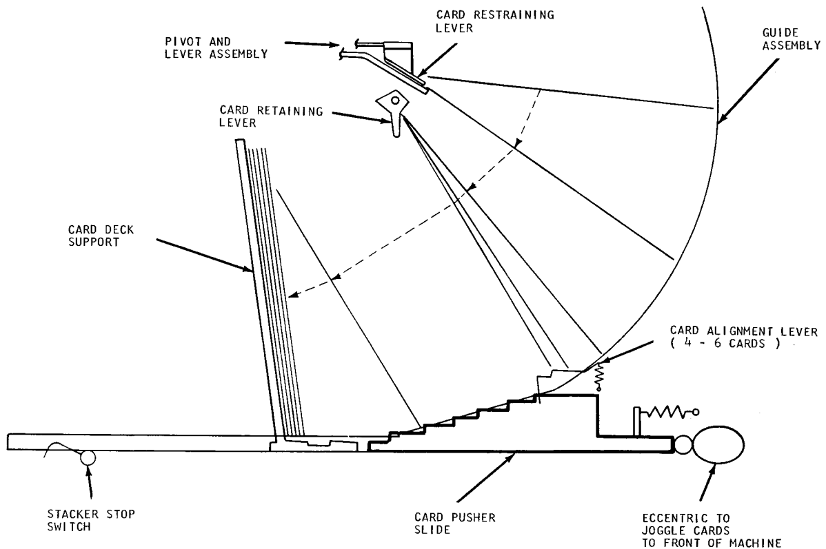
Figure 23. Stacker Schematic
