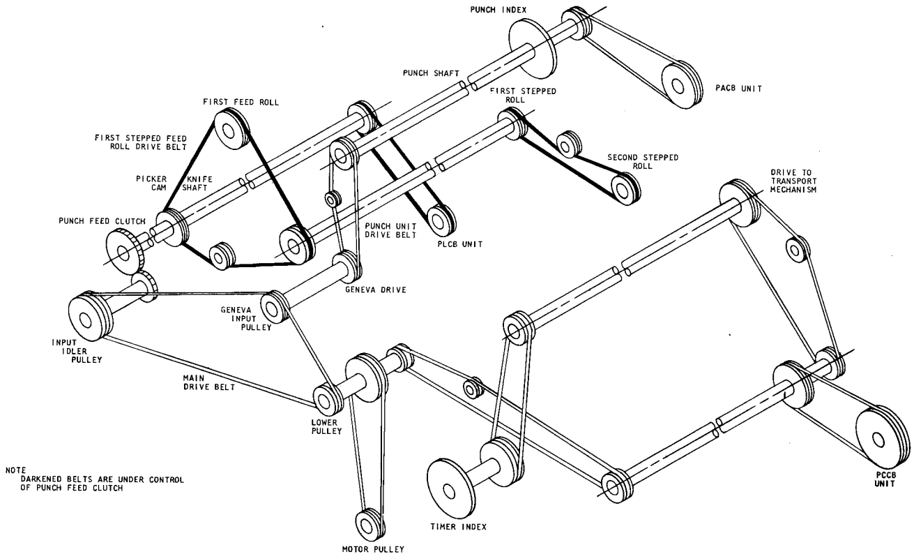
Figure 26. Punch Feed Timing Belts
