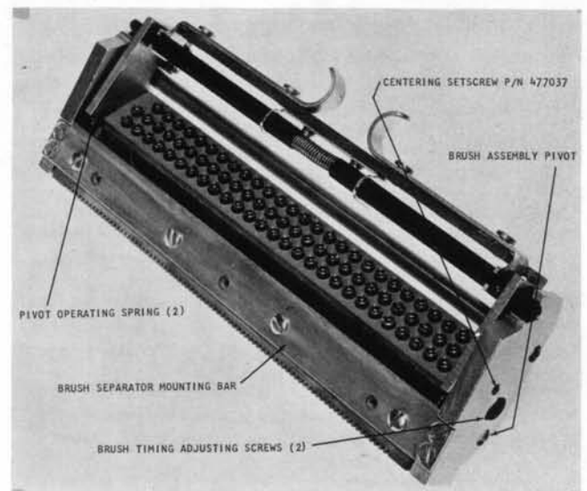
Figure 18. Brush Assembly
