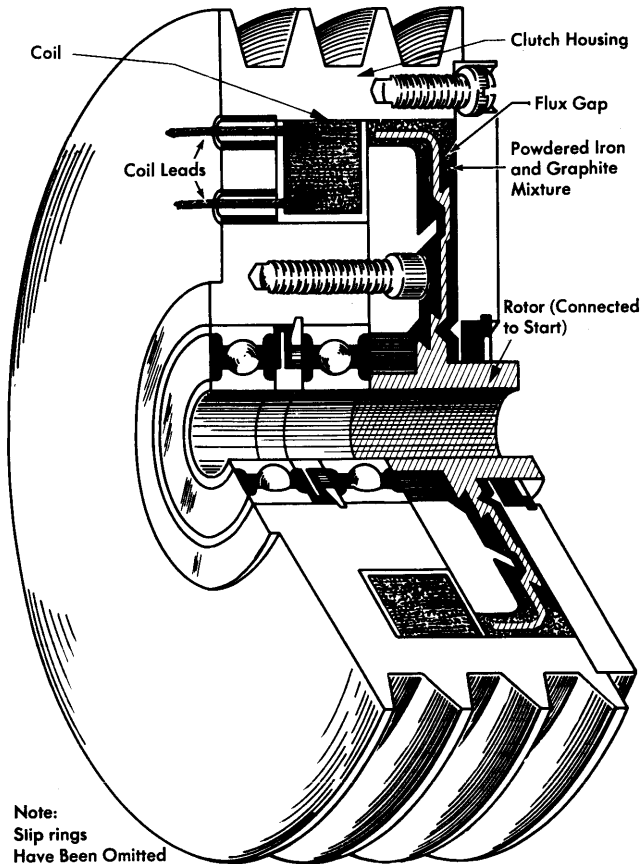
Figure 53. Magnetic Clutch
