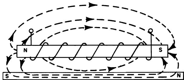
Figure II-52. Magnetic-Head Principles
