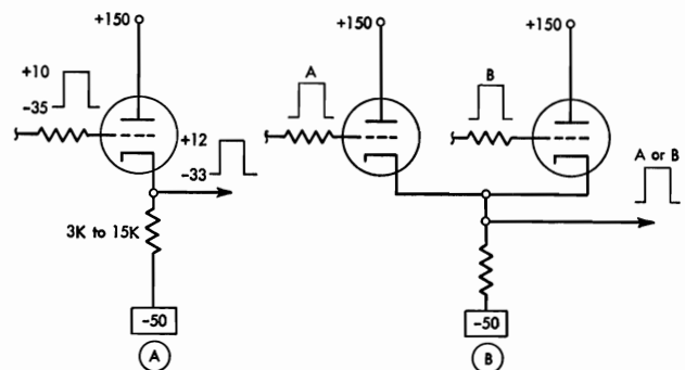
Figure II-10. Cathode Followers
