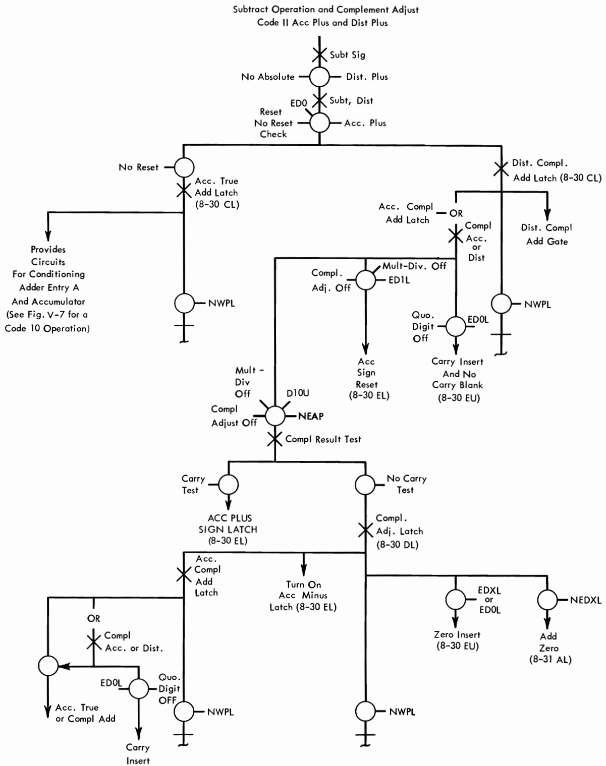
Figure V-10. Subtract and Complement Adjust
