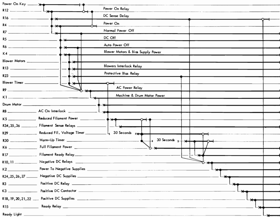
Figure IX-2. Power-On Sequence
