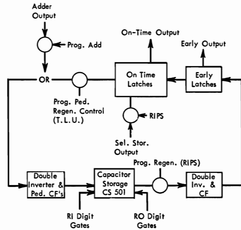
Figure III-1. Data Flow for Program Register
