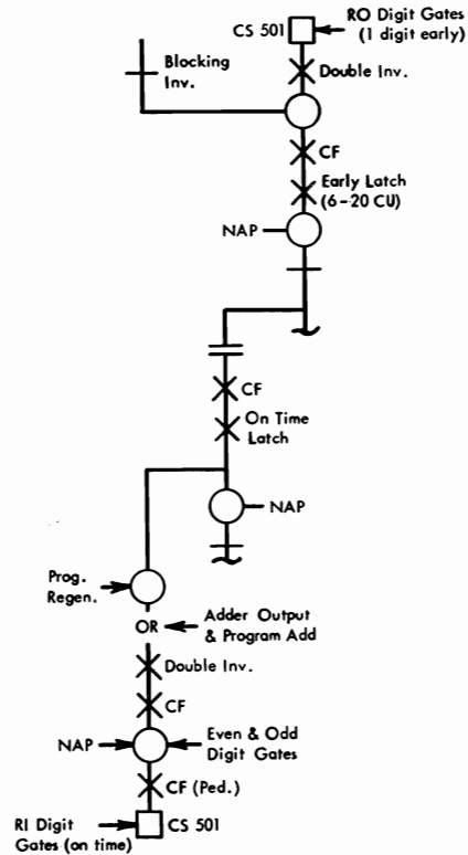
Figure III-2. Regeneration of Program Register
