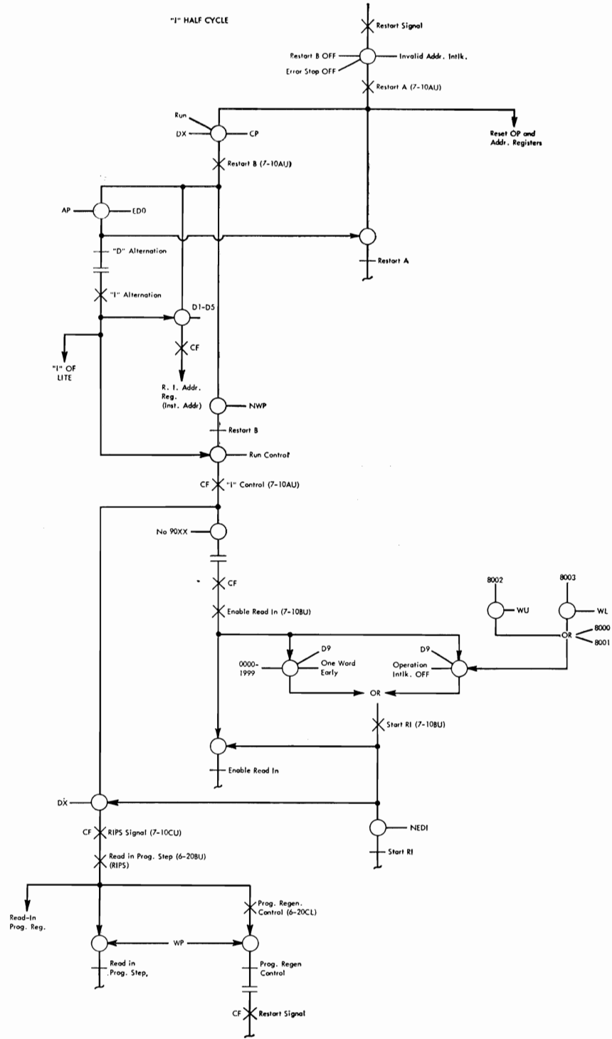
Figure V-2. I1 Half Cycle
