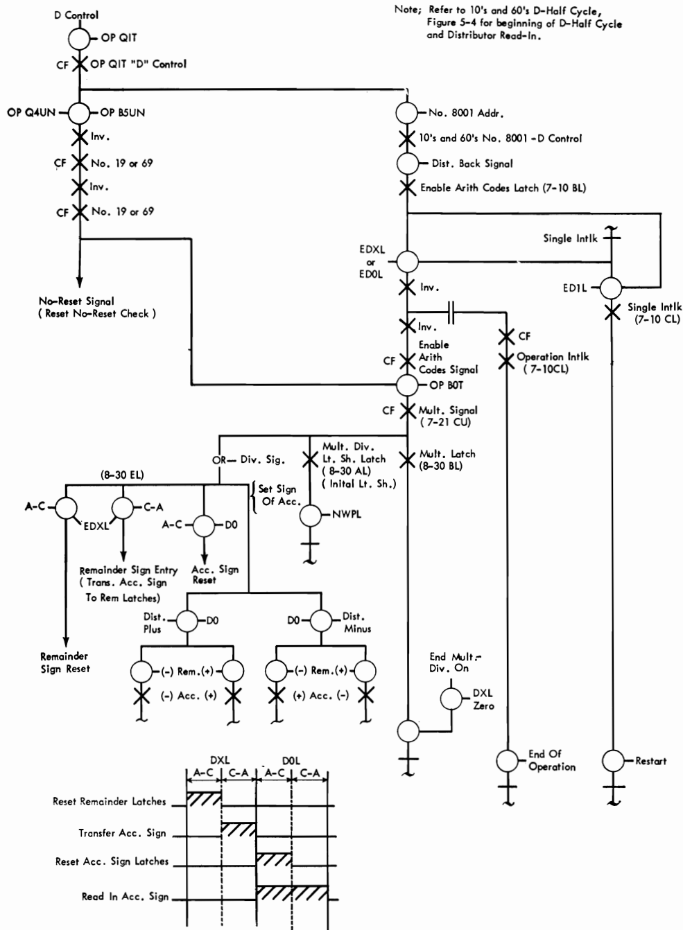
Figure V-37. Multiply Setup
