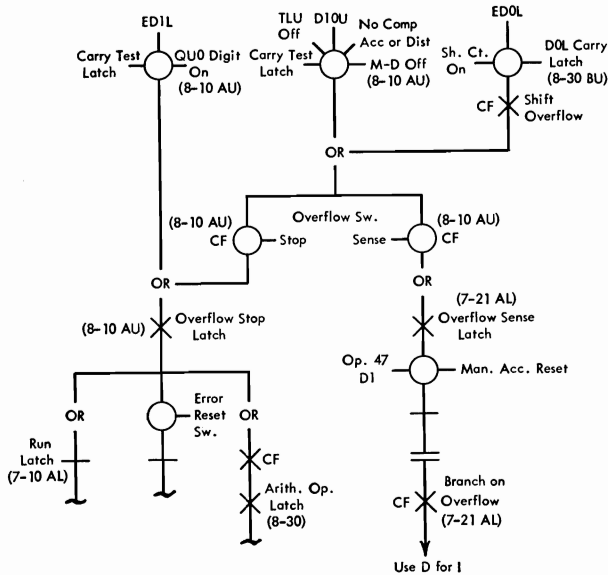
Figure III-5. Overflow Sense-Stop
