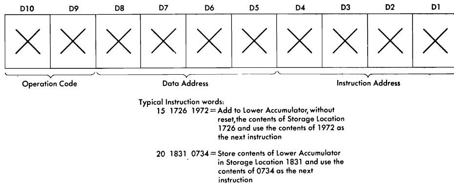
Figure I-10. Instruction Word Meaning
