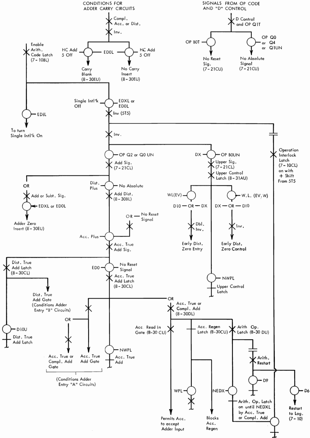
Figure V-7. Add Upper Function Chart—Code 10
