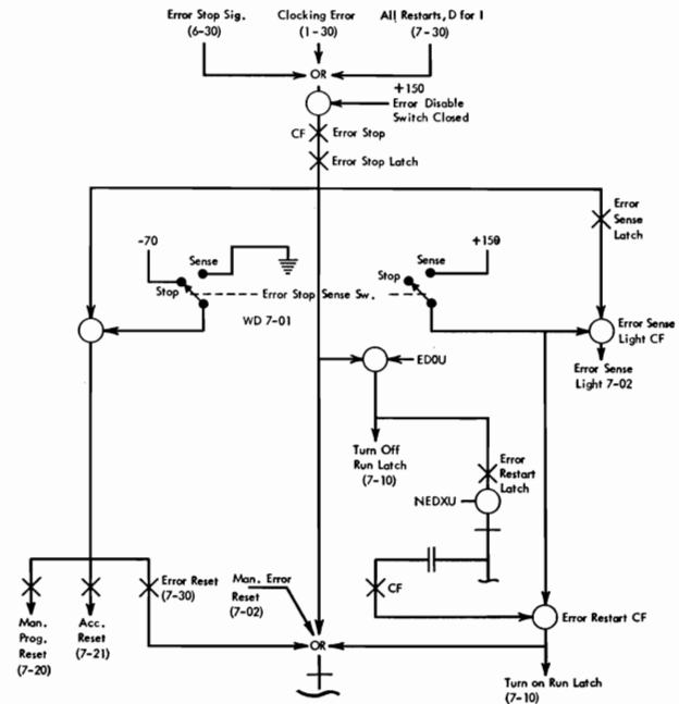
Figure III-7. Error Stop and Sense Function Chart
