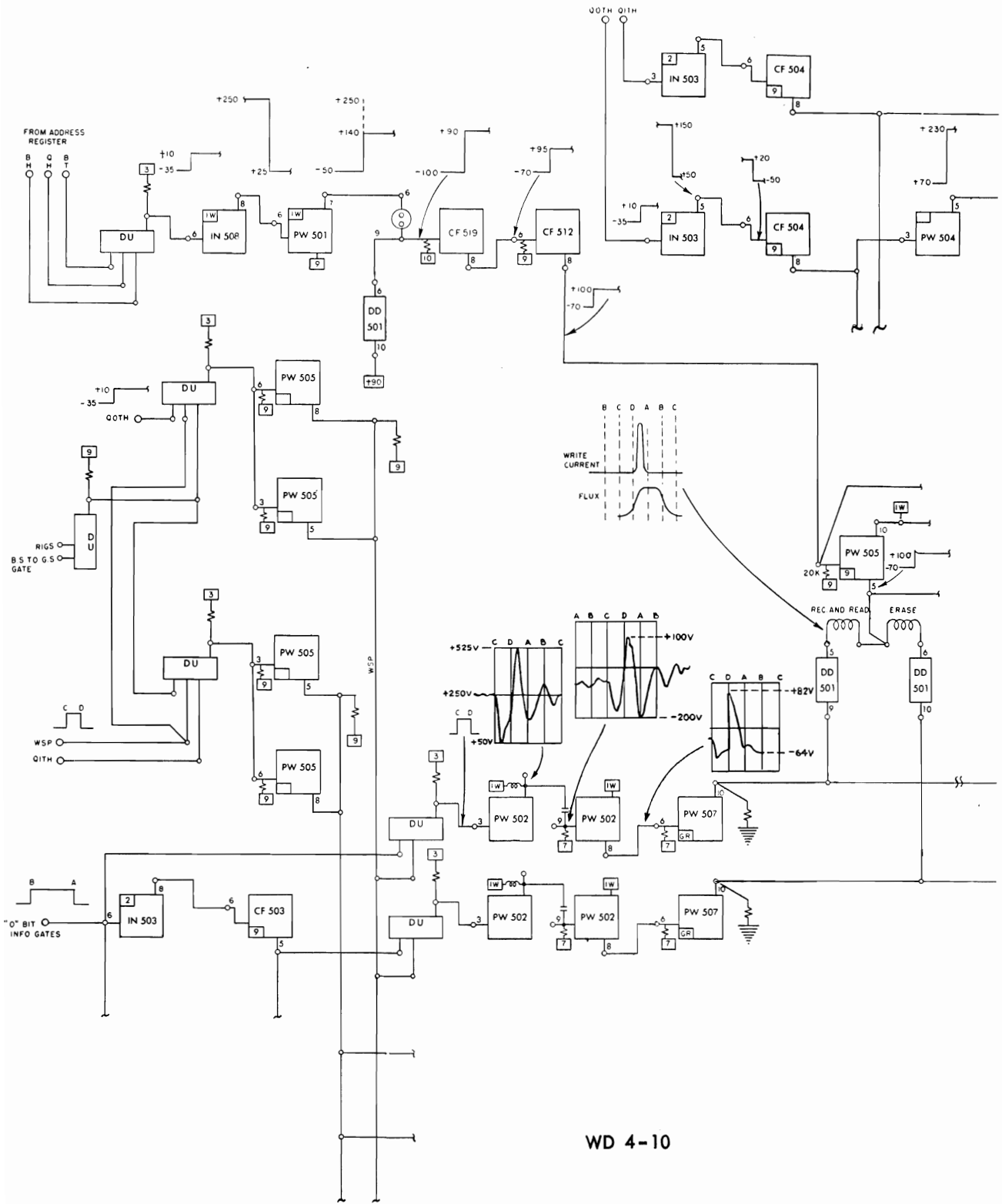
Figure II-62. General Storage Head Connection and Read-Write Circuitry
