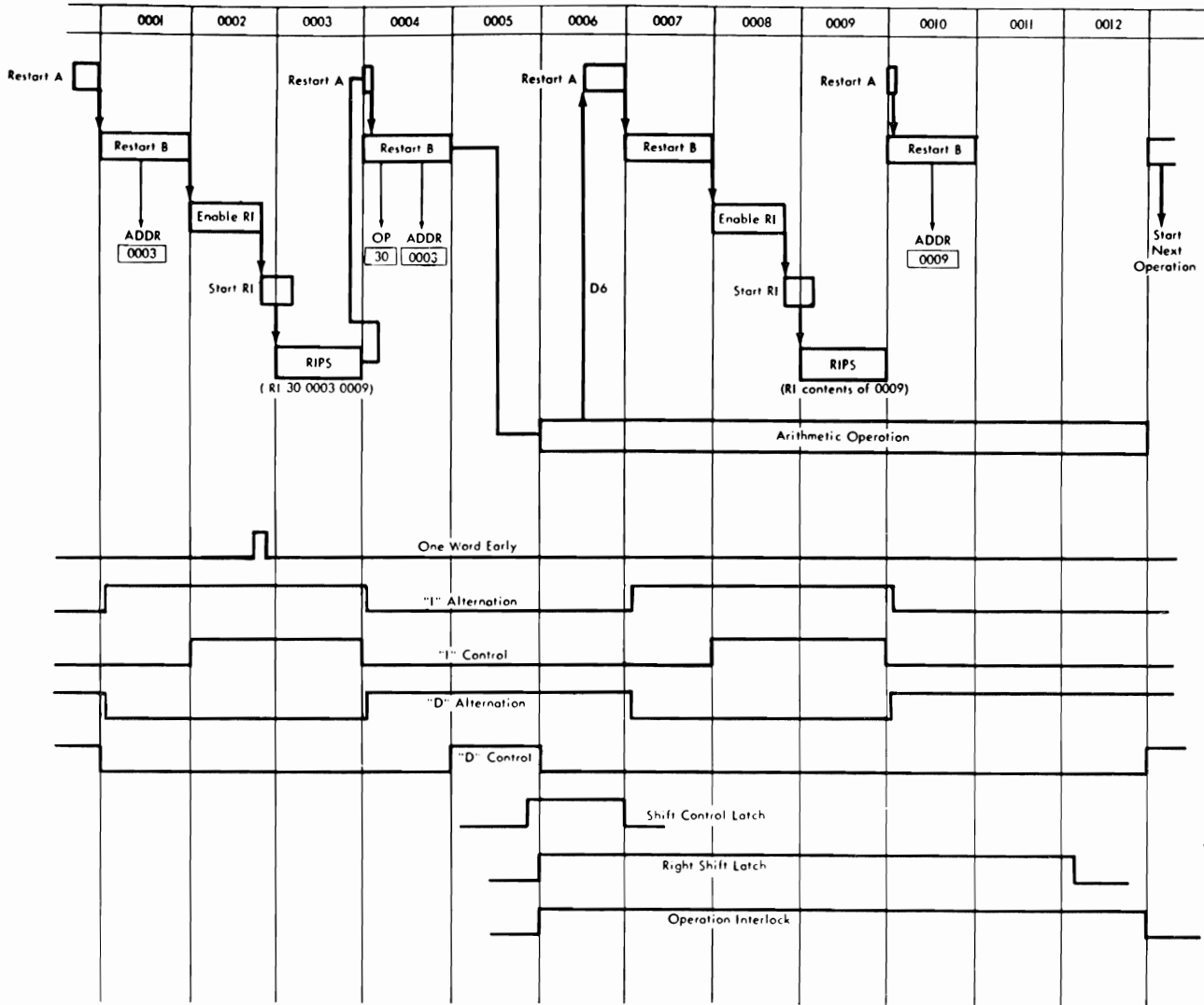
Figure V-20. Control Commutator Operation—Code 30
