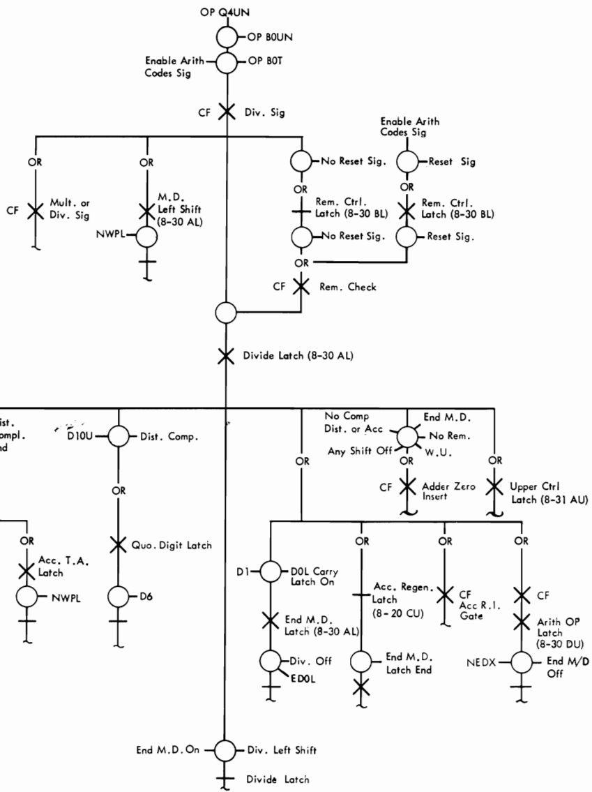
Figure V-46. Divide Controls
