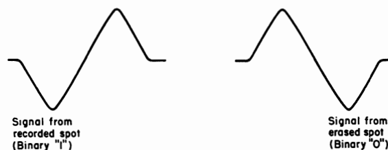
Figure II-56. Read Signals
