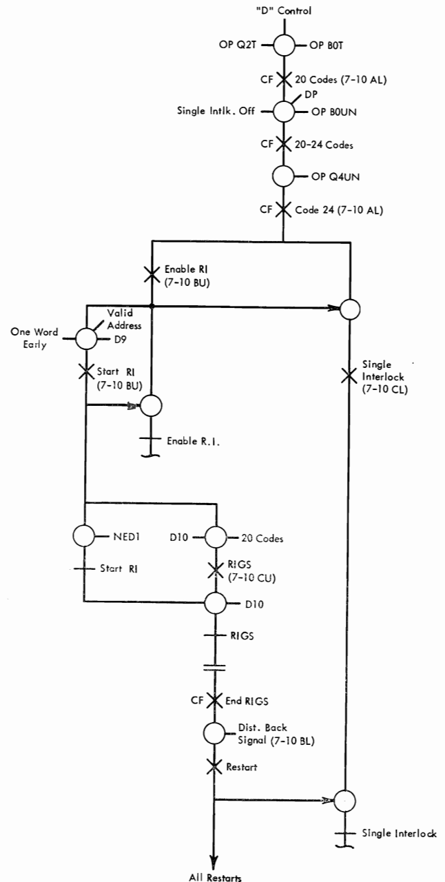
Figure V-19. Store Distributor—Code 24
