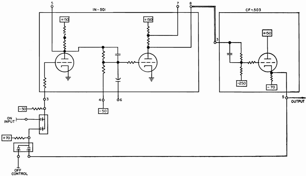
Figure II-19. Latch Circuit
