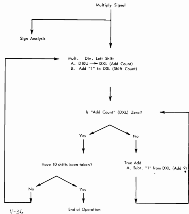
Figure V-36. Multiplication—Code 19
