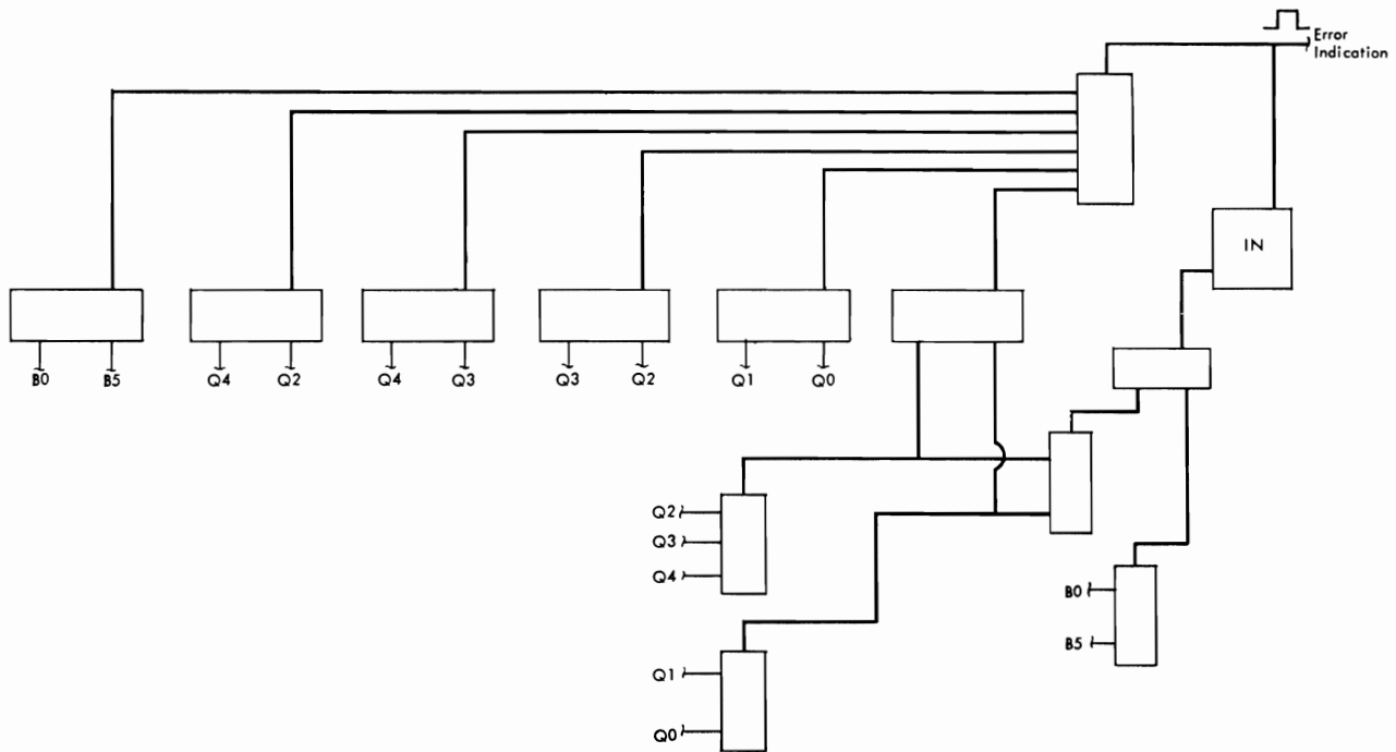
Figure II-69. Validity Check Schematic
