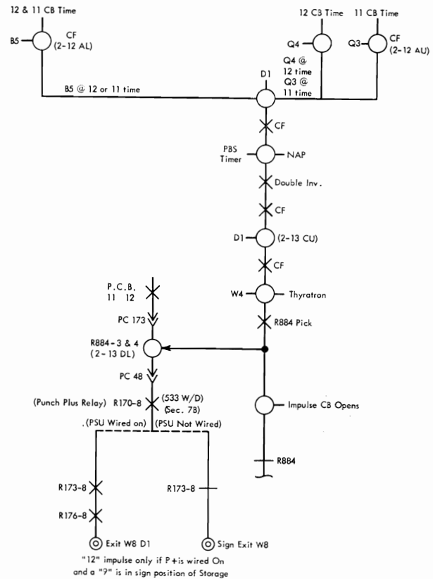
Figure VII-10. Sign Punch-Out—Word 8
