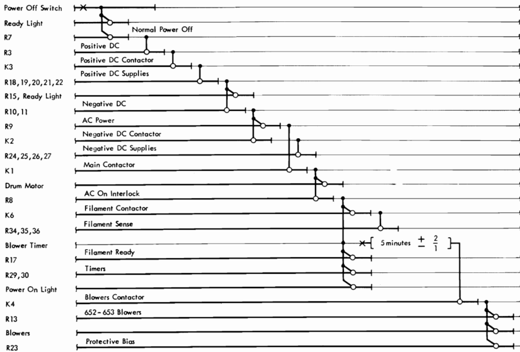
Figure IX-3. Power-Off Sequence
