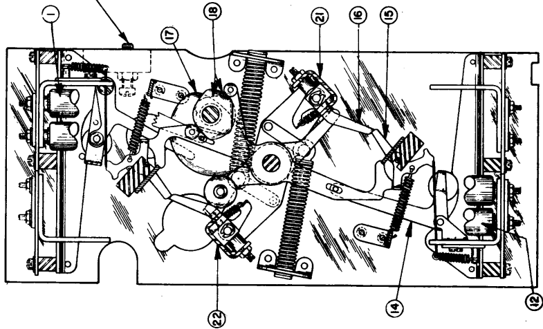
RESTORING MECHANISM
